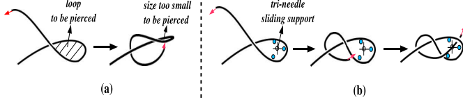
Fig. 7. (a): After a loop has been created, it is not guaranteed that its size will be maintained during further manipulation (b): Passive/static sliding supports (tri-needle) is used to maintain the size of the loops to be pierced in future.
