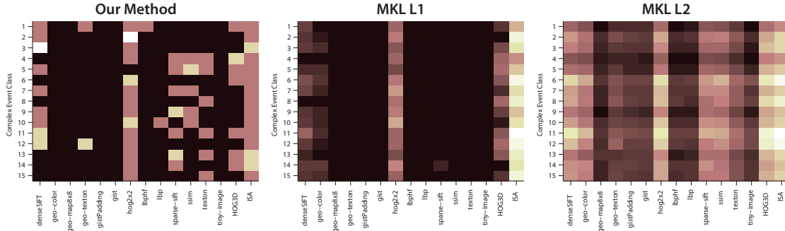
Figure 7. Visualizations of the feature combinations learned by various methods for each of the complex event classes. The matrix visualizes the weights learned for each of the features. Lighter colors correspond to higher weights. Class numbers are given in Tables 1 and 2.
