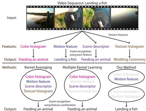
Figure 1. Compared to standard methods for feature combination, our method performs feature selection (grayed features) and considers sets of features independently (separate bubbles). This allows us to select the right features to use and correctly recognize the video sequence as “Landing a fish”.
