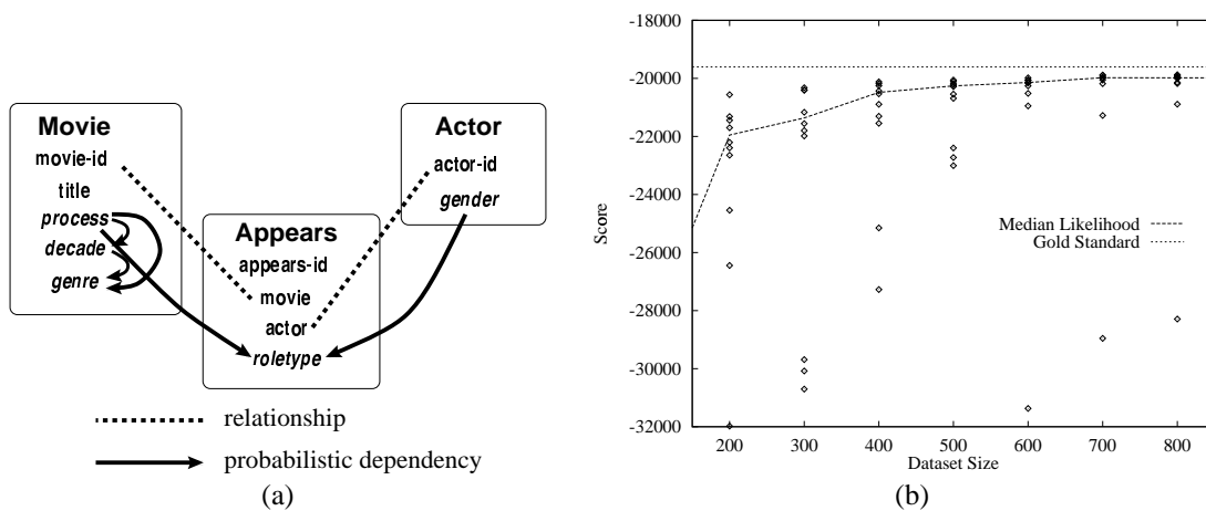
Figure 2: (a) The PRM learned for the movie domain, a real-world database containing about 11000 movies and 7000 actors. (b) Learning curve showing the generalization performance of PRMs learned in the genetic domain. The x -axis shows the databases size; the y -axis shows log-likelihood of a test set of size 10,000. For each sample size, we show 10 independent learning experiments. The curve shows median log-likelihood of the models as a function of the sample size.
