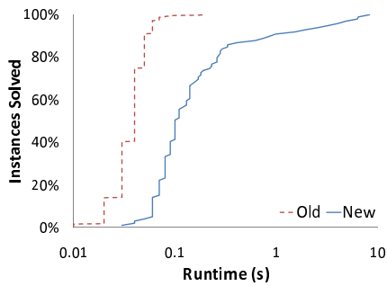
Fig. 32. Matching (test data, 1000 bids/256 goods)
