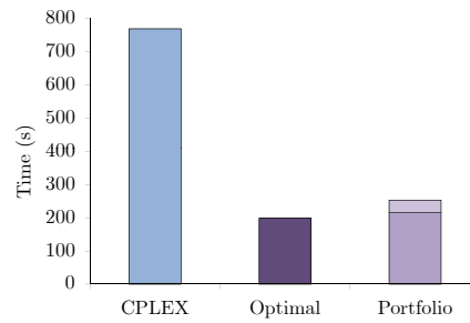
Fig. 23. Portfolio Runtimes (test data, 1000 bids/256 goods).
