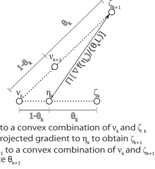
Figure 1. Schematic view of Algorithm 1
