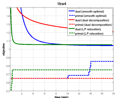
Figure 4. Typical optimization curves showing both the (original) dual objective and the decoded integer solution. Compared are our smooth-optimal method, the dual decomposition method of Komodakis & Paragios (2009) and the LP relaxation algorithm of Globerson & Jaakkola (2007).
