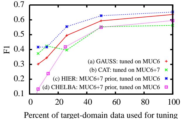
Figure 3: Adding a relevant HIER prior helps compared to the GAUSS baseline ((c) > (a)), while simply CAT’ing or using CHELBA can hurt ((d) \approx (b) < (a)), except with very little data), and never beats HIER ((c) > (b) \approx (d)).
