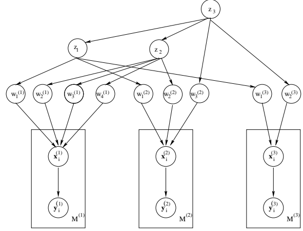
Figure 2: Graphical representation of the hierarchical transfer model.
