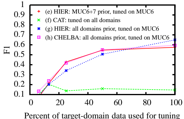
Figure 4: Transfer aware priors CHELBA and HIER effectively filter irrelevant data. Adding more irrelevant data to the priors doesn't hurt (( e ) \approx ( g ) \approx ( h )), while simply CAT'ing it, in this case, is disastrous (( f ) \ll ( e )). ological corpora (UT & YAPEX), labeled not with person names but with protein names instead, along with the CSPACE e-mail and MUC7 news article corpora. The robustness of our prior prevents a model trained on all five domains ( g ) from degrading away from the intra-genre, same-task baseline ( e ), unlike the model trained on concatenated data ( f ). CHELBA ( h ) performs similarly well in this case, perhaps because the domains are so different that almost none of the features match between prior and tuning data, and thus CHELBA backs-off to a standard \mathcal{N}(0, 1) prior.
