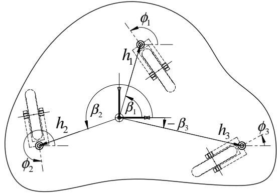
Figure 3: Powered Caster Vehicle Geometry
