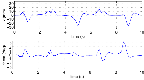
Figure 11: Positions without dynamic compensation
