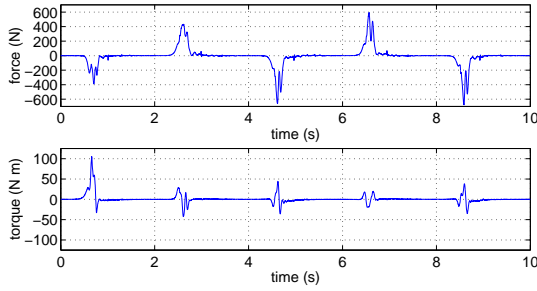
Figure 10: Dynamic compensation force- x and dynamic compensation torque- \theta
