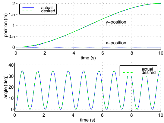
Figure 13: Base x and y positions vs. time and PUMA joint 1 angle vs. time
