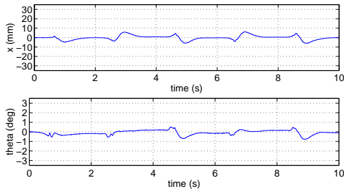
Figure 12: Positions with dynamic compensation
