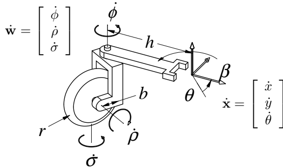
Figure 4: Powered Caster “Manipulator”
