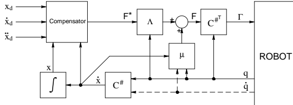
Figure 7: Controller Schematic
