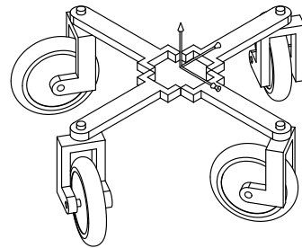
Figure 5: Cooperating powered caster manipulators
