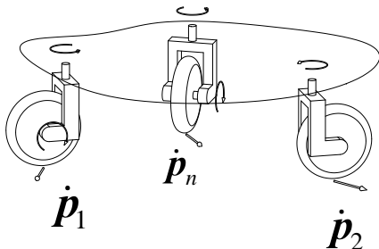
Figure 6: Contact point velocities
