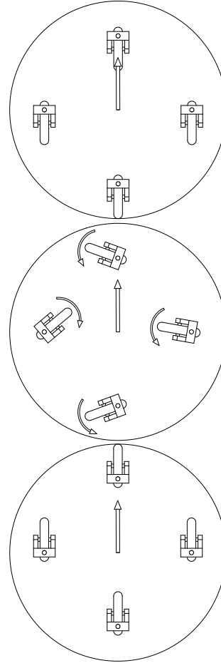
Figure 9: Wheel “flip” during y -axis motion which leads to large dynamic disturbance forces
