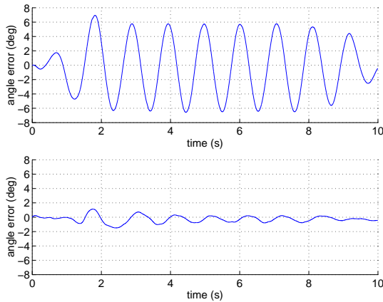
Figure 15: Base orientation error without and with dynamic compensation
