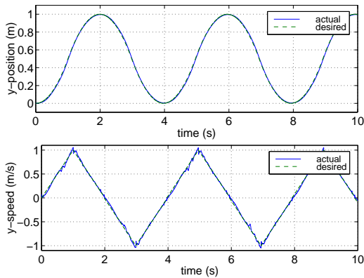
Figure 8: Position vs. time and velocity vs. time with dynamic compensation
