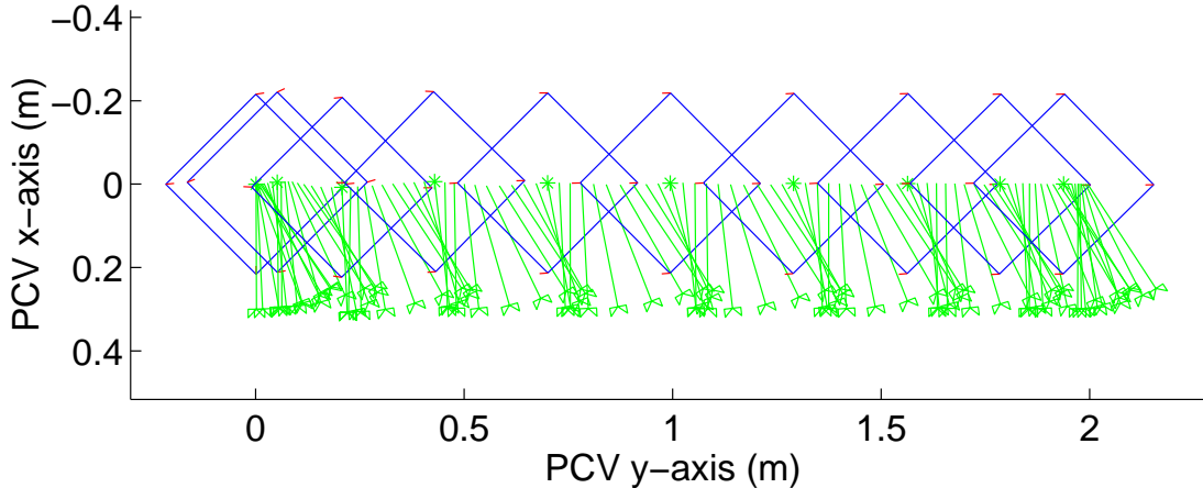
Figure 14: Path of robot and manipulator arm
