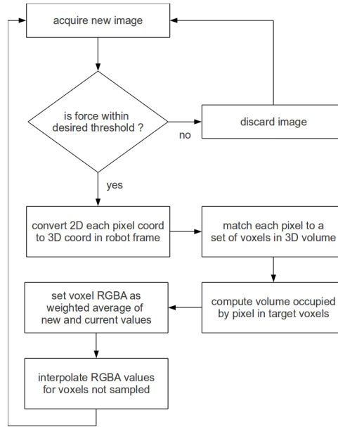
Fig. 8. 3D reconstruction dataflow.
