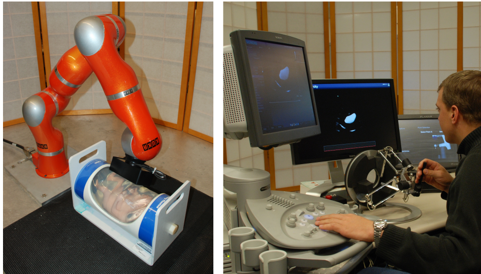
Fig. 3. Overall system: (Left) LWR robot manipulator examining phantom model of a foetus. (Right) Master User Console composed of the ultrasound imaging system (US) with 3D visualization and 6-DOF haptic interface.
