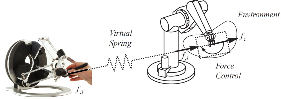
Fig. 4. Teleoperation approach with a virtual spring and force control. The desired force, f_d , is produced by the virtual spring based upon the position difference between the master and slave robot end-effectors. The force controller on the slave robot enforces the contact force, f_c , to track this desired force while the desired force is fed back to the user at the master device.
