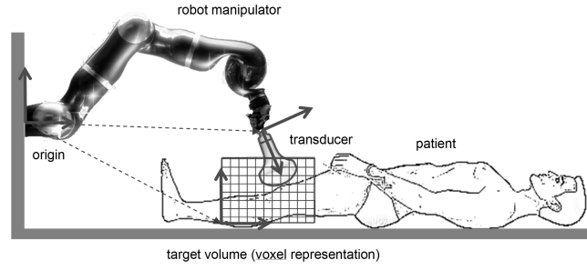
Fig. 7. The target volume defines the anatomical area when the scan occurs. Streaming 2D images are acquired from the transducer and inserted into the 3D voxel representation.
