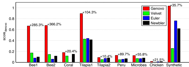
FIG. 2. The numbers above the bars represent the improvement (in percentages) between Genovo and the second-best method. To compute \text{score}_{denovo} , we had to complete each list of contigs to a full assembly, by mapping each read to the location that explains it best. Reads that did not align well to any location were treated as singletons—aligned perfectly to their own contig. We could not run EULER-SR on Coral, and the corresponding entry is missing from all figures.
