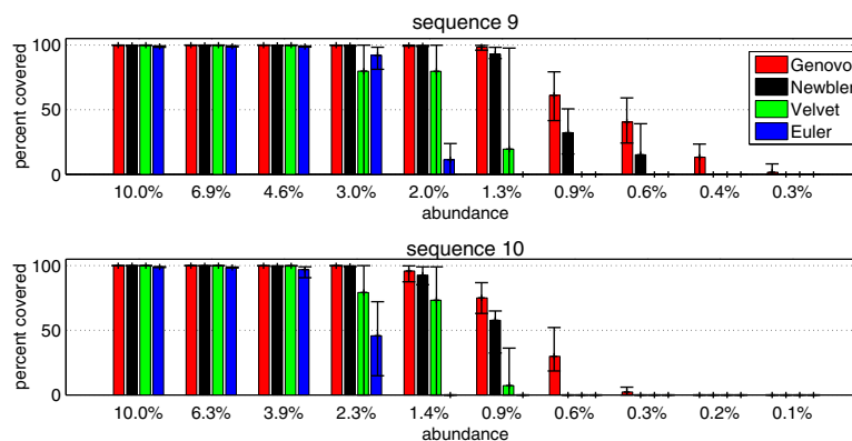
FIG. 5. 50k simulated reads were extracted from 10 sequences in 10 experiments. Abundance levels were different in each experiment, starting from uniform and getting more and more extreme. The graph shows the mean percentage of bases that were covered from the two least abundant sequences across the 10 experiments, as their abundance got worse. Error bars represent the minimum and maximum numbers obtained in 5 replicates. The full set of results across all abundances and all sequences is given in the Supplementary Material.
