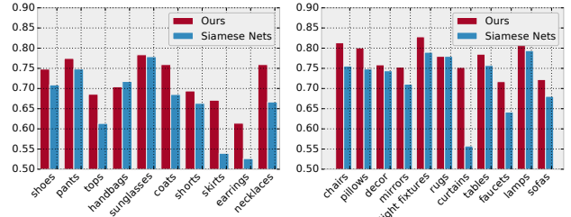
Figure 1. Accuracy per category. Left: STL-Fashion, right: STL-Home.
