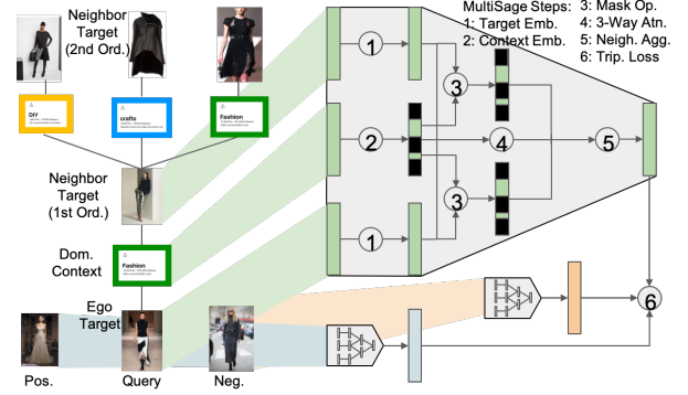
Figure 4: The overall neural architecture of MULTISAGE.
