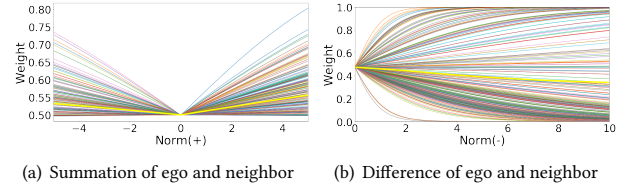
Figure 6: Attention over different self-neighbor pairs.
