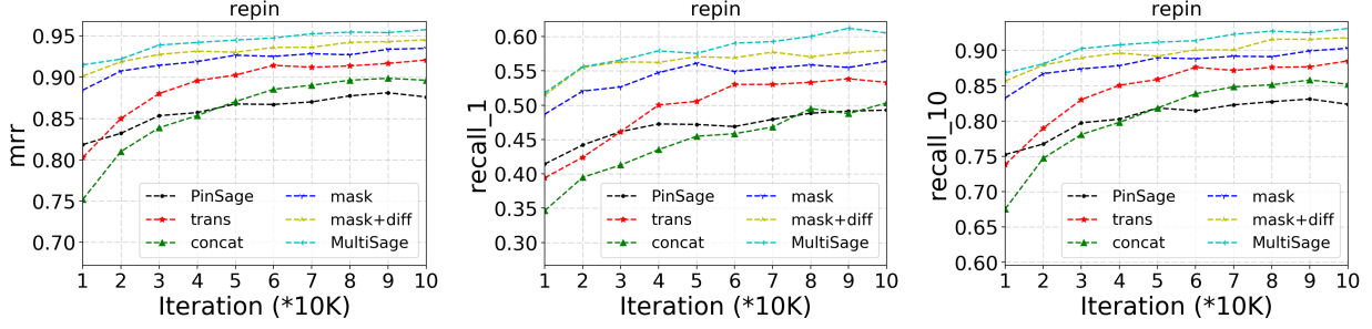
Figure 5: Performance of different model variants on Pinterest . Scores are computed every 10K iterations on the testing data.
