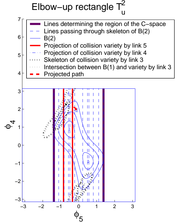
Fig. 5. The path (drawn as red dashed line) projected to T_u^2 . The two triangles pointed to the left and right represent the initial and goal configurations, respectively
