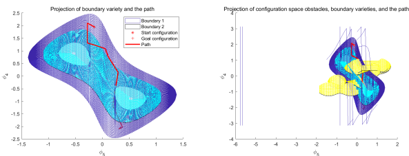
Fig. 8. (a): Projection of the C-space; (b): Projection of \mathcal{C}_{\text{obst}}
