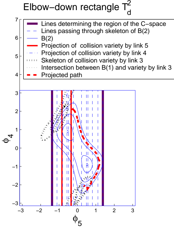
Fig. 6. The path (drawn as red dashed line) projected to T_d^2 .
