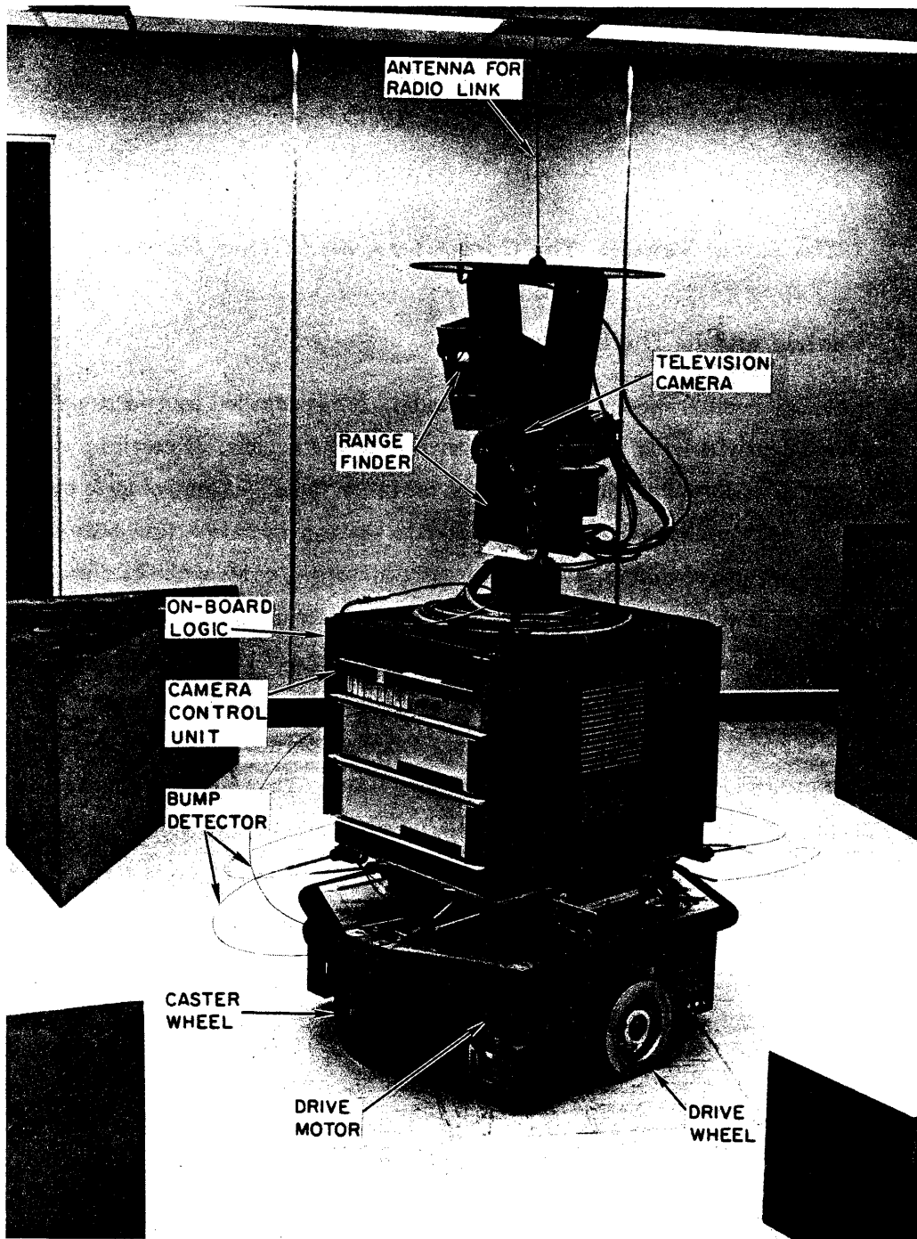
Figure 1: AUTOMATON VEHICLE*
