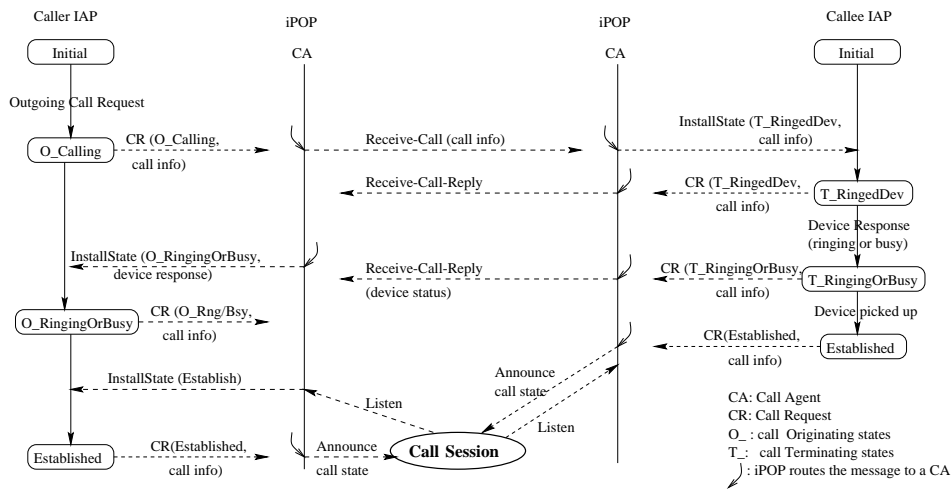
Fig. 2. Call Session Establishment
